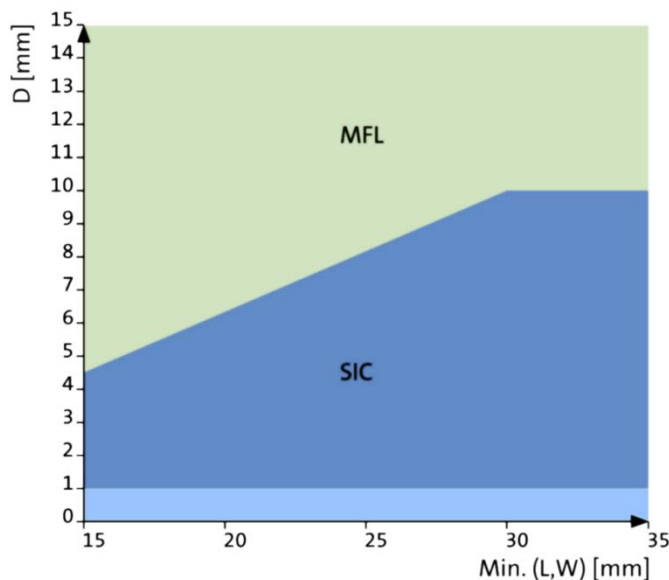
Figure 3: Optimal sizing regimes of the MFL and SIC inspection methods for internal metal loss defects depicted for a 15 mm wall thickness. The green and blue areas indicate the favored sizing regimes of these two techniques, respectively. The light blue area in the figure illustrates that for a feature depth less than 1 mm the Probability of Detection (POD) with metal loss characterization is smaller than 90%. (L = length, W = width, D = depth of feature.)
