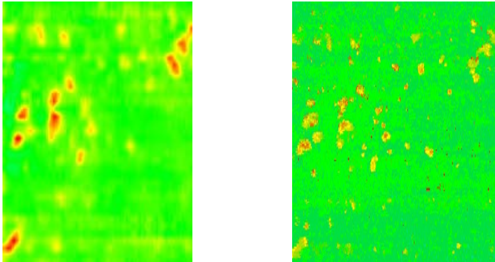
Figure 6: Top of line corrosion in a test pipeline. The left panel shows inspection results obtained with a SIC tool, the right figure represents data derived from an automatic UT measurement. Corrosion patterns in both excerpts can easily be correlated.
