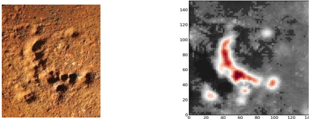
Figure 5: (left) Pitting corrosion in a steel plate. (right) The corresponding data made with a SIC sensor in a laboratory setup with sample spacing of 2 mm in both directions and a specific pseudo-lift-off scaling (all values in mm).
