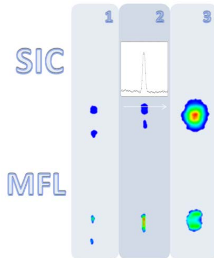
Figure 4: Defect patterns are shown twice, as SIC pseudo-lift-off (top) and MFL field strength (bottom) data, respectively. The vertical lanes differentiate the test features, which were made in a 16" joint with 12.6 mm wall thickness: (lane no. 1) 2 bore holes with 10 mm diameter each and edge-to-edge separation of 40 mm in circumferential direction of the pipe, (no. 2) like the previous lane, but bores with edge-to-edge separation of 20 mm, and (no. 3) a bore hole with a diameter of 35 mm. The inset shows a SIC raw signal trace, i.e. before conversion to pseudo-lift-off scale, whereas its positions in the c-scan are indicated by the white arrow.
