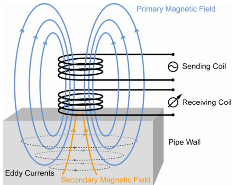
Figure 2: Schematic sketch of coil system for measuring metal loss.
