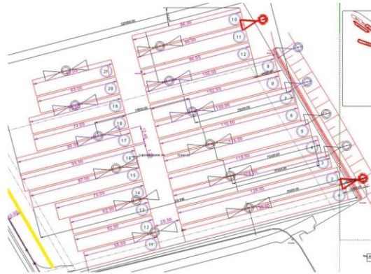
Figure 9: A typical yard layout with router/repeater masts
