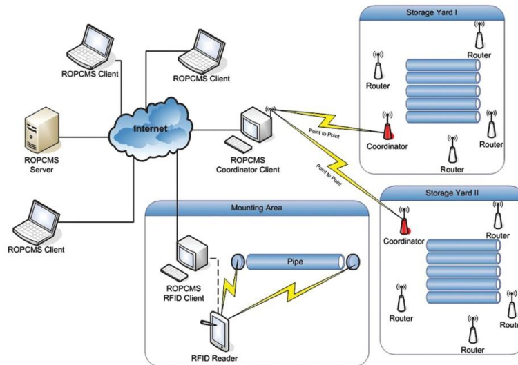
Figure 11: Central Control System ROPCMS
