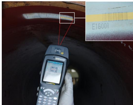
Figure 8: transmission of pipe number from barcode to RFID chip
