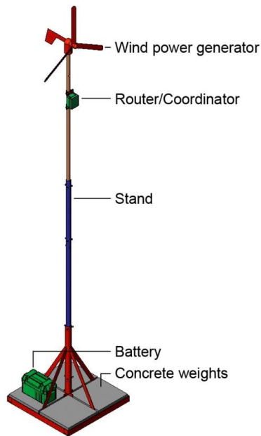
Figure 10: Self-sufficient router/repeater system
