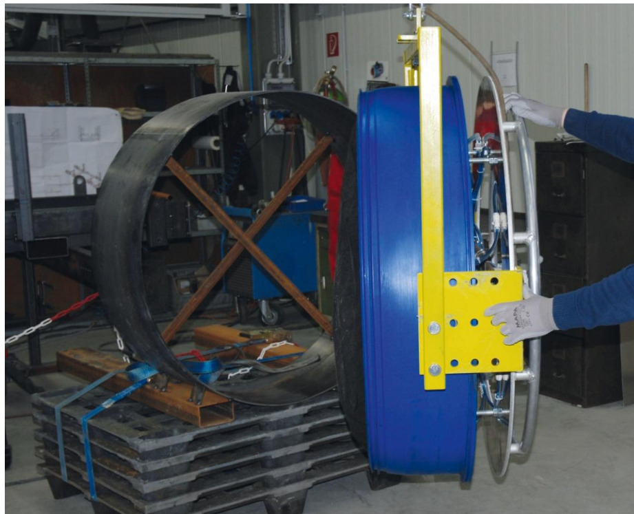
Figure 2: Internal cap mounting device
