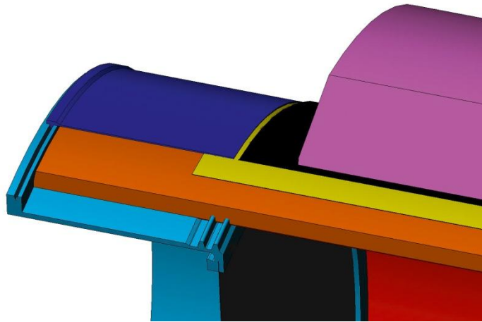
Figure 6: Outer cap with inner cap ziplock system
