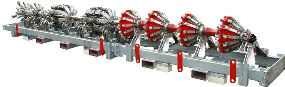
Figure 3: ROSEN 14"/18" multi-diameter MFL tool
