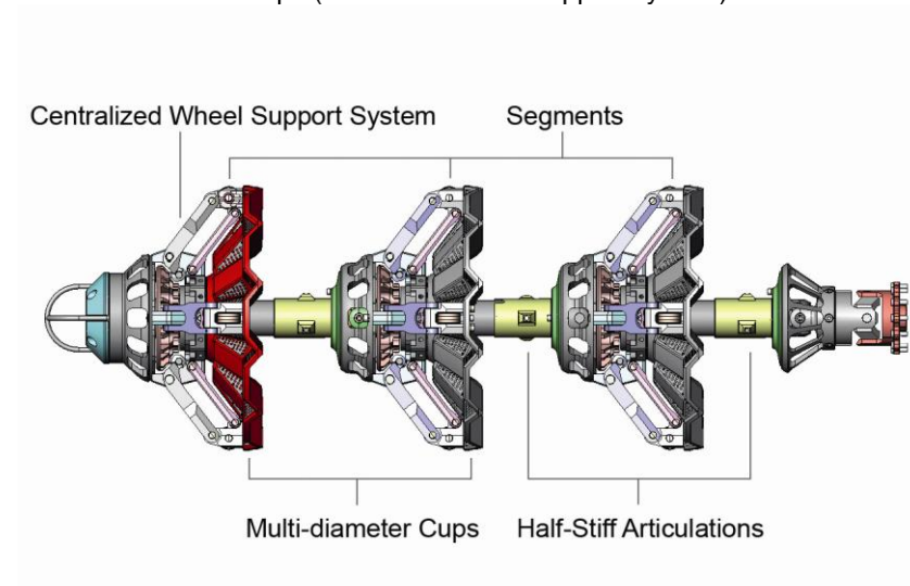
Figure 4: Drawing of the 14"/20" pull unit
